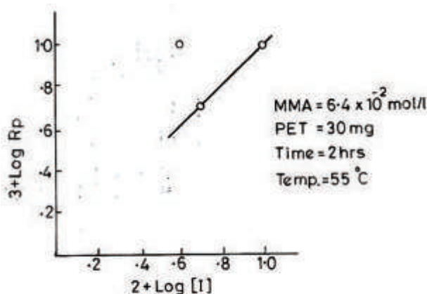
FIG. 2. GRAPH BETWEEN LOG RATE OF POLYMERIZATION AND LOG CONCENTRATION OF INITIATOR
