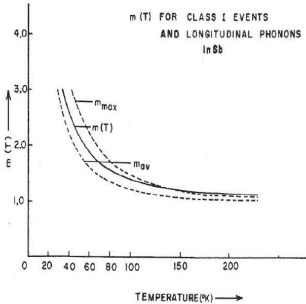
Figure - 2 : m(T) for class- I events for longitudinal phonons in InSb. m_{max} is the upper bound given by Guthrie while m_{av} is the average value of upper and lower bounds of Guthrie.
