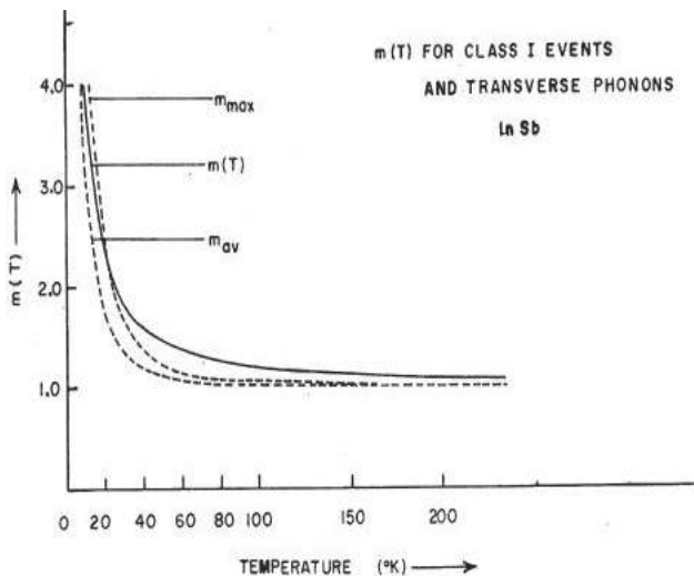
Figure - 3 : m(T) for class - I events for transverse phonons in InSb. m_{max} is the upper bound given by Guthrie while m_{av} is the average value of upper and lower bounds of Guthrie.
