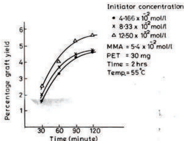
FIG. 1. GRAPH BETWEEN PERCENTAGE GRAFT YIELD AND POLYMERIZATION TIME
