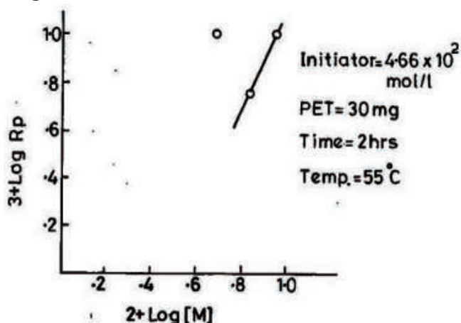
FIG.4: GRAPH BETWEEN LOG RATE OF POLYMERIZATION AND LOG CONCENTRATION OF METHYL METHACRYLATE
