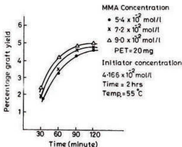
FIG. 3. GRAPH BETWEEN PERCENTAGE GRAFT YIELD AND POLYMERIZATION TIME
