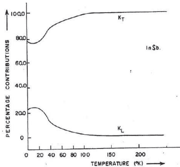
Figure-5: Percentage contribution of transverse and longitudinal phonons in InSb. K_T is the percentage contribution of transverse phonons while K_L is the percentage contribution of longitudinal phonons.
