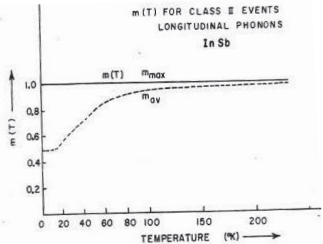
Figure - 4 : m(T) for Class - II events for longitudinal phonons in InSb. m_{max} is the upper bound given by Guthrie which is same as m(T) . m_{av} is the average value of upper and lower bounds of Guthrie.
